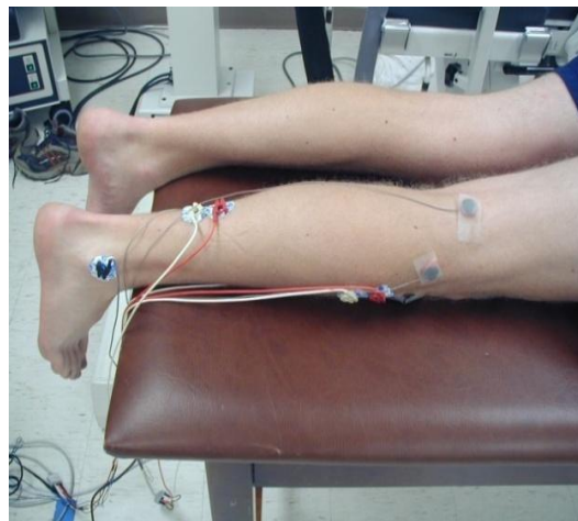
Figure 2 – Electrodes placement for Spinal Reflex Testing
